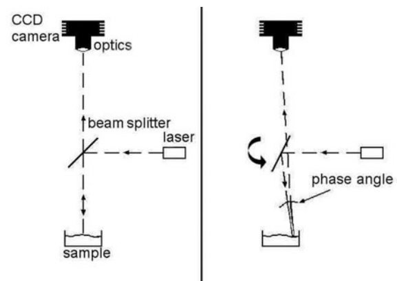
Fig. 1. The small-angle laser goniometer. Retroreflection from the sample is observed through the beam-splitter by the charge-coupled device (CCD) camera (left). Non-zero phase angles (source–target–detector) are obtained by rotating the beam-splitter (right). The distance from beam-splitter to sample was 12 cm, and from the CCD to the sample 120 cm.
