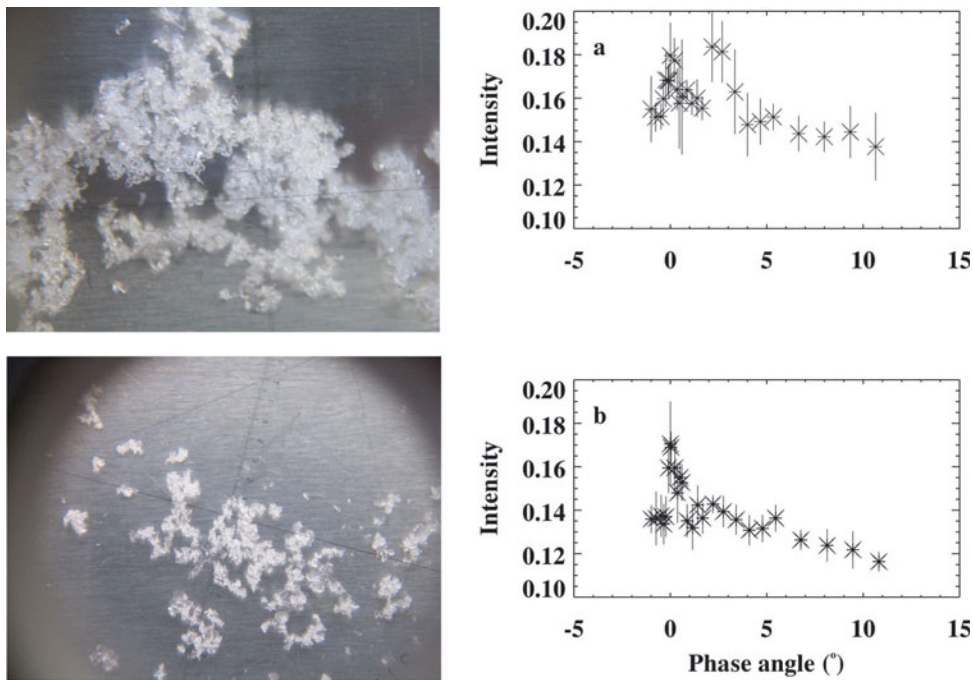
Fig. 9. Effect of grain-size: (a) 0.2–0.5 mm surface grains from previous day's snowfall (8 March 2005) and (b) 0.1–0.3 mm surface grains from previous day's snowfall (8 March 2005; same sample as shown in Fig. 7b).
