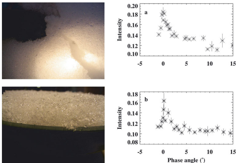
Fig. 2. Refrozen layers from the 2004 campaign measured (a) below (11 March 2004) and (b) above 0^{\circ}\text{C} (19 March 2004).
