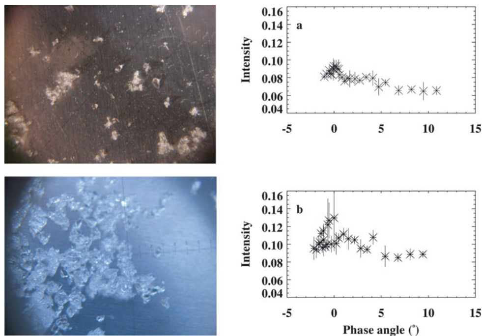
Fig. 6. (a) Refrozen (rounded) grains (same sample as shown in Fig. 5b) and (b) grains of a coarser structure taken from 40 cm depth in the snowpack (also measured on 3 March 2005). The difference in the smoothness of the phase curve is visible (cf. also Fig. 9).
