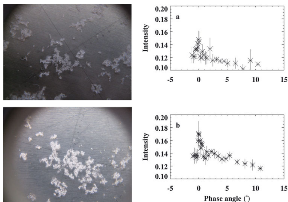
Fig. 7. Effect of compression on surface (needle) grains: (a) slightly compressed (7 March 2005) and (b) compressed overnight (8 March 2005).
