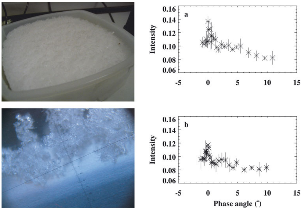
Fig. 4. (a) Melting grains (same sample from 2 March 2005 as shown in Fig. 3a) and (b) same sample after refreezing. The millimeter scale visible in the bottom left image is the same in all the grain images.
