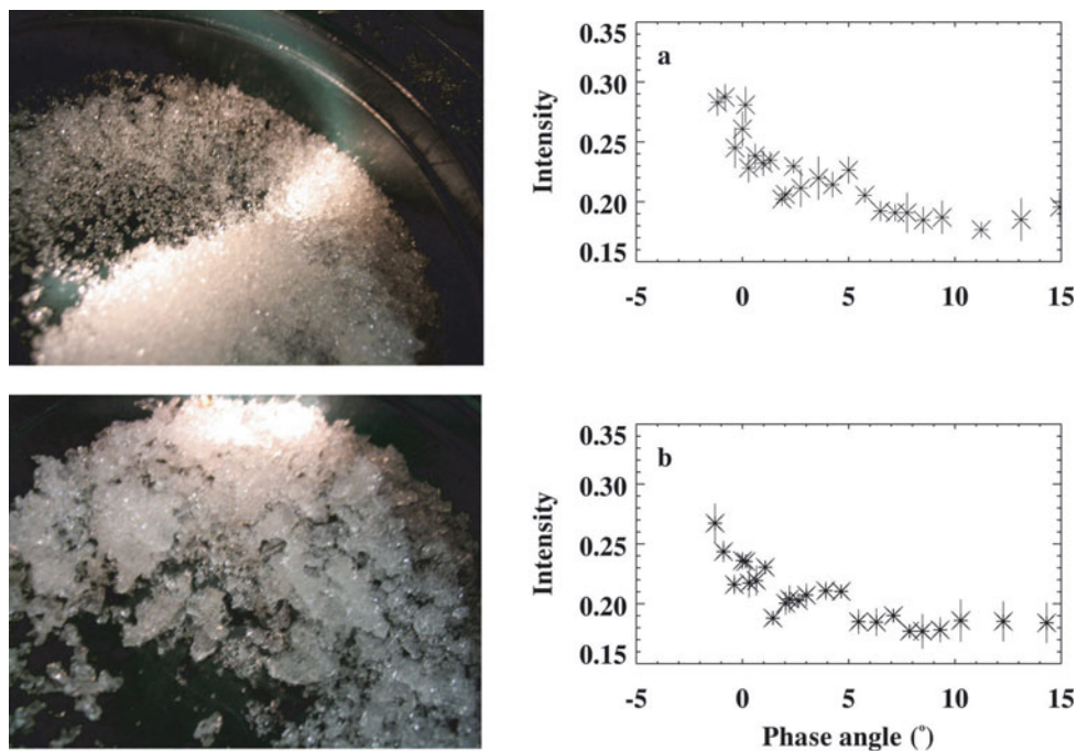
Fig. 11. Comparison with data from 2004: (a) aged snow from about 40 cm depth in the snowpack and (b) depth hoar from 60 cm depth in the snowpack. The samples (both measured on 23 March 2004) are photographed in a sample cup of about 11 cm diameter.
