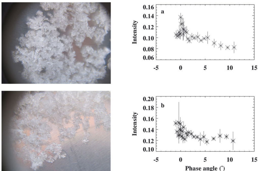
Fig. 3. (a) Melting and (b) frozen surface grains measured on 2 March 2005. The grain images were taken with a millimeter scale (more clearly visible in the bottom left image in Fig. 4).
