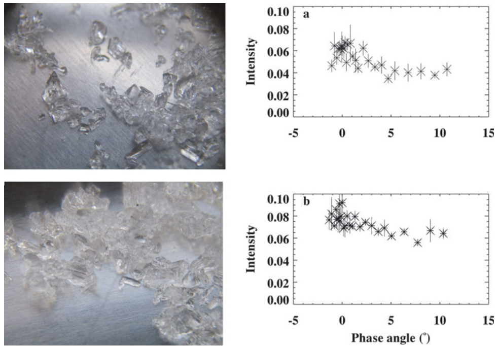
Fig. 10. Larger grain sizes (than those shown in Figs 8 and 9): (a) depth hoar with grains of 2 mm from about 80 cm depth in the snowpack (4 March 2005) and (b) a similar sample with grains of 2–3 mm (10 March 2005).
