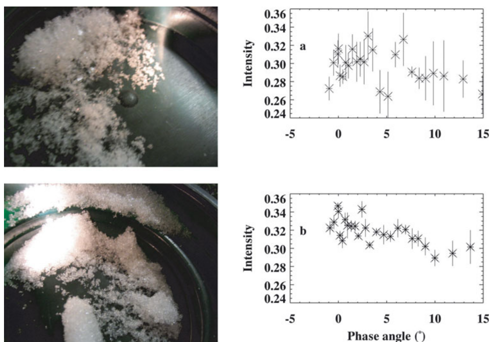
Fig. 12. Data from 2004 measurements: (a) new snow from the surface and (b) aged snow from about 20 cm depth in the snowpack (both samples measured on 23 March 2004). The effect of rounded grain structure (compared with fresh fallen grains of a finer structure) on the smoothness of the phase curve is also clear in this case. The sample grains are photographed in a sample cup of about 11 cm diameter.
