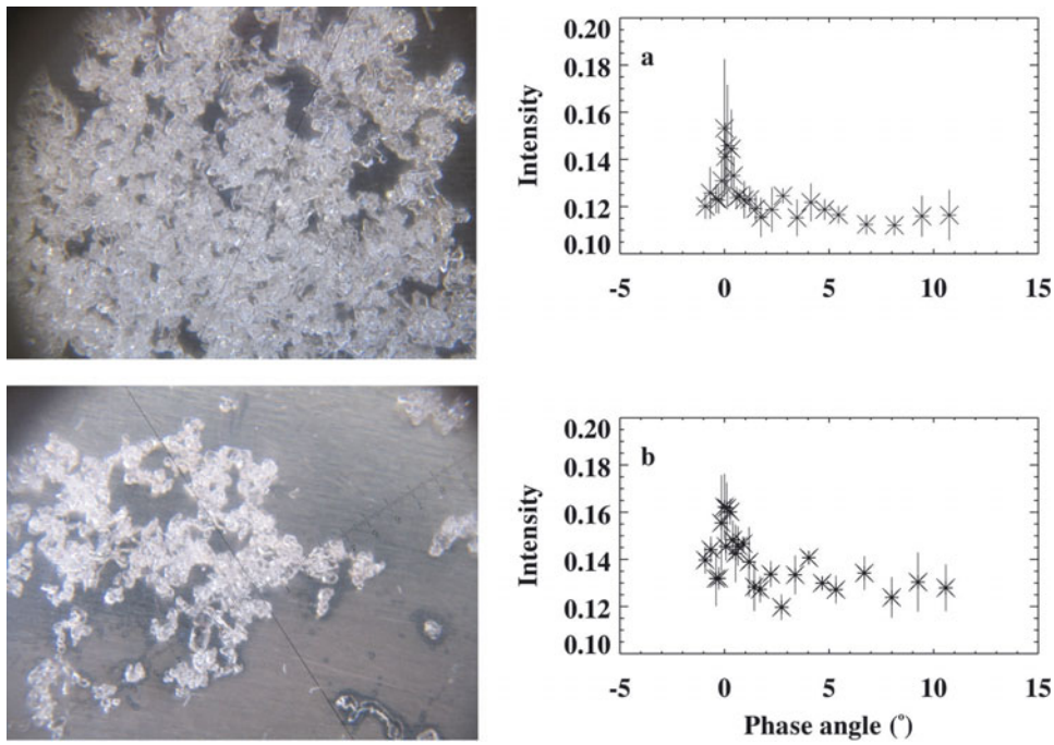
Fig. 8. Comparison of the effect of grain size: (a) 0.7–1.0 mm rounded grains from 5–10 cm depth in the snowpack (12 March 2005) and (b) same sample slightly melted and refrozen (13 March 2005).
