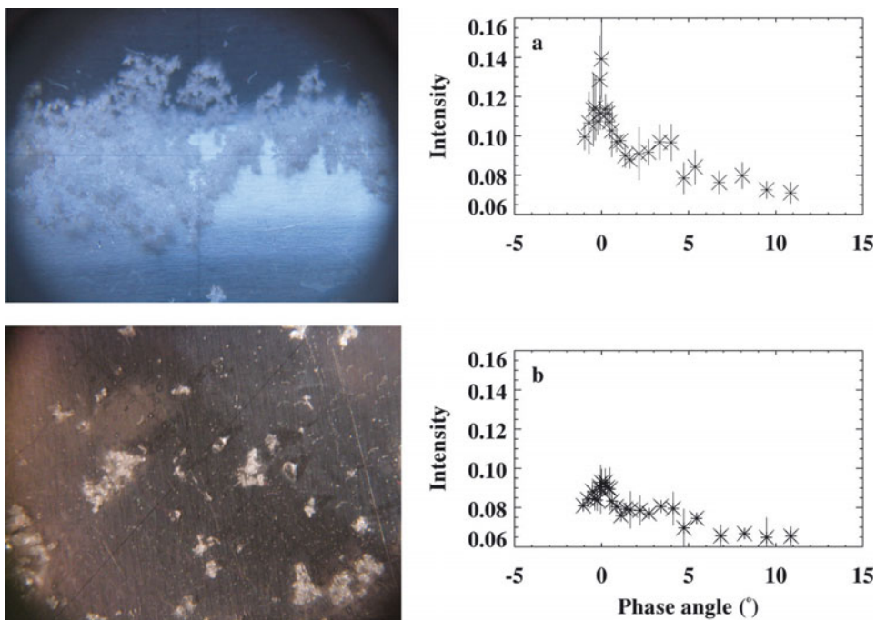
Fig. 5. (a) Melting new snow produces a stronger backscatter effect than does (b) the refrozen sample (both from 3 March 2005). Both surfaces were tilted to eliminate the effect of specular reflection.
